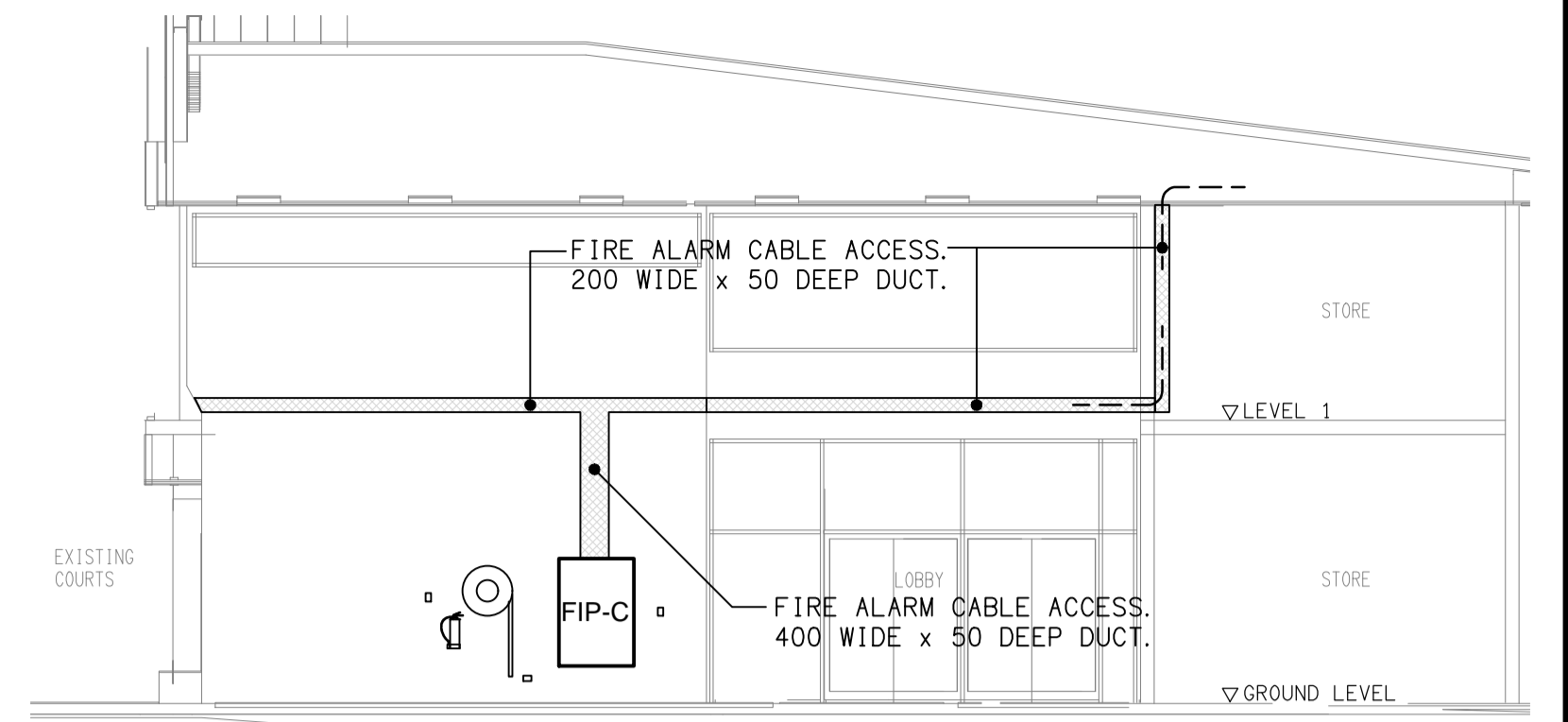
DETAIL A FIRE ALARM CABLE ACCESS DUCT SECTION SCALE: 1:100
